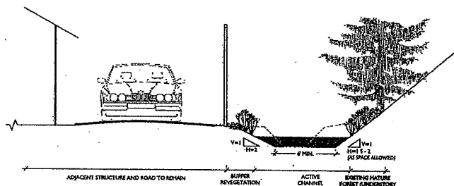
TYPICAL CHANNEL SECTION IN AREA 3
