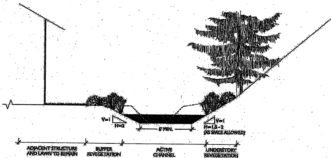
Figure 11. Channel improvements in Area B
