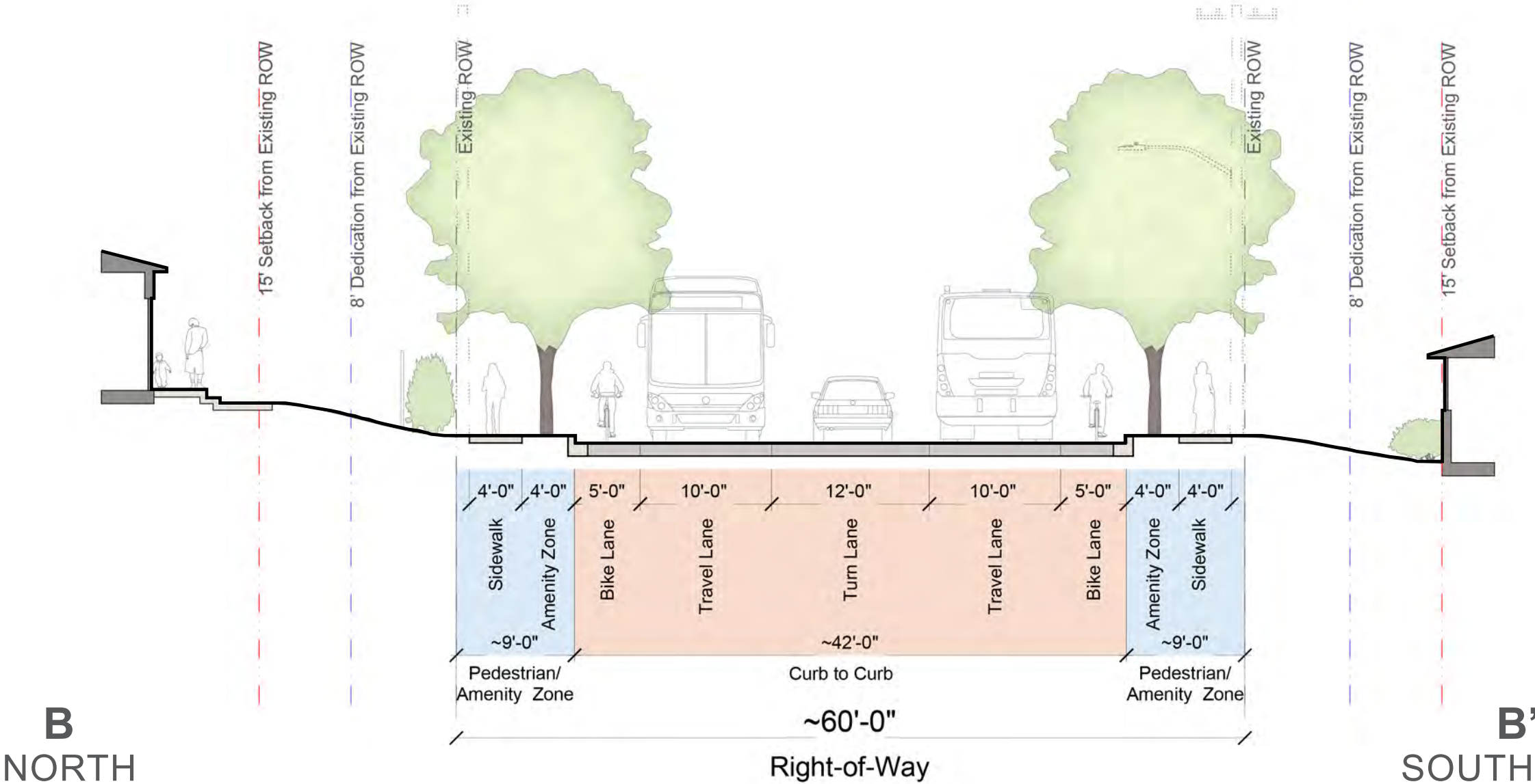
SECTION B EXISTING CONDITIONS
