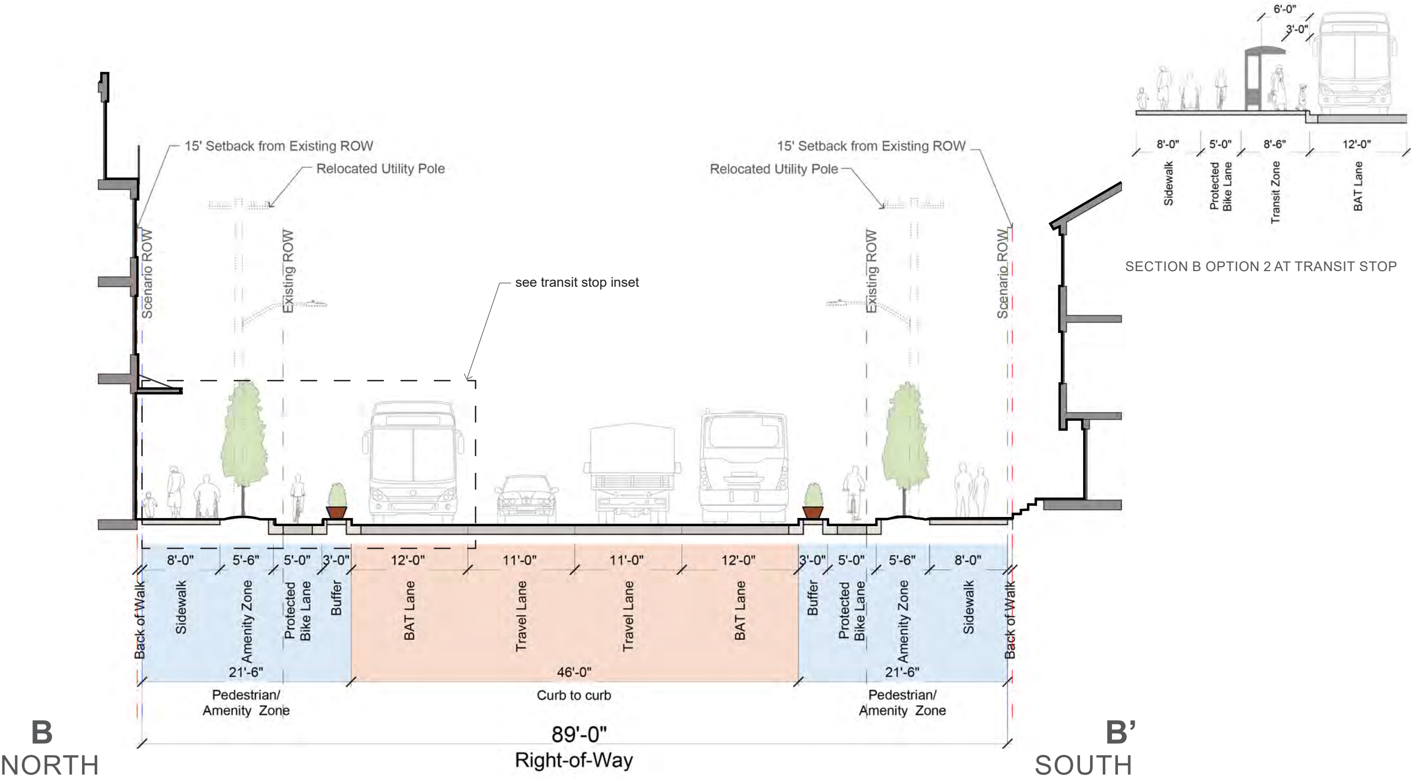
SECTION B OPTION 2
