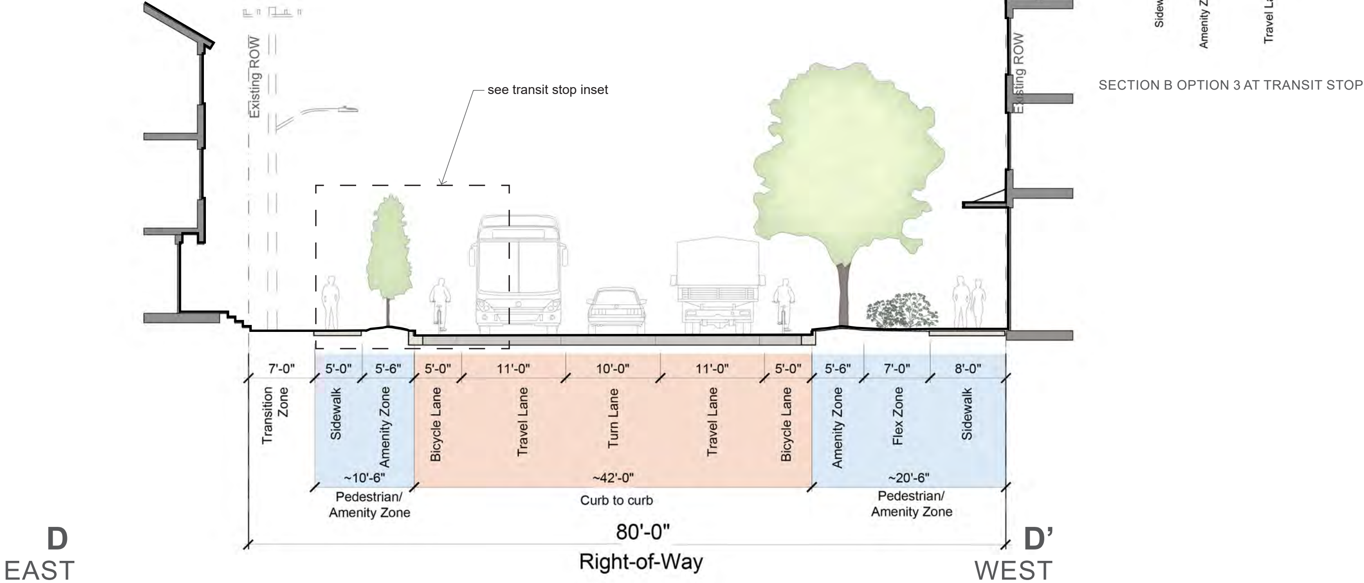
SECTION D OPTION 3
