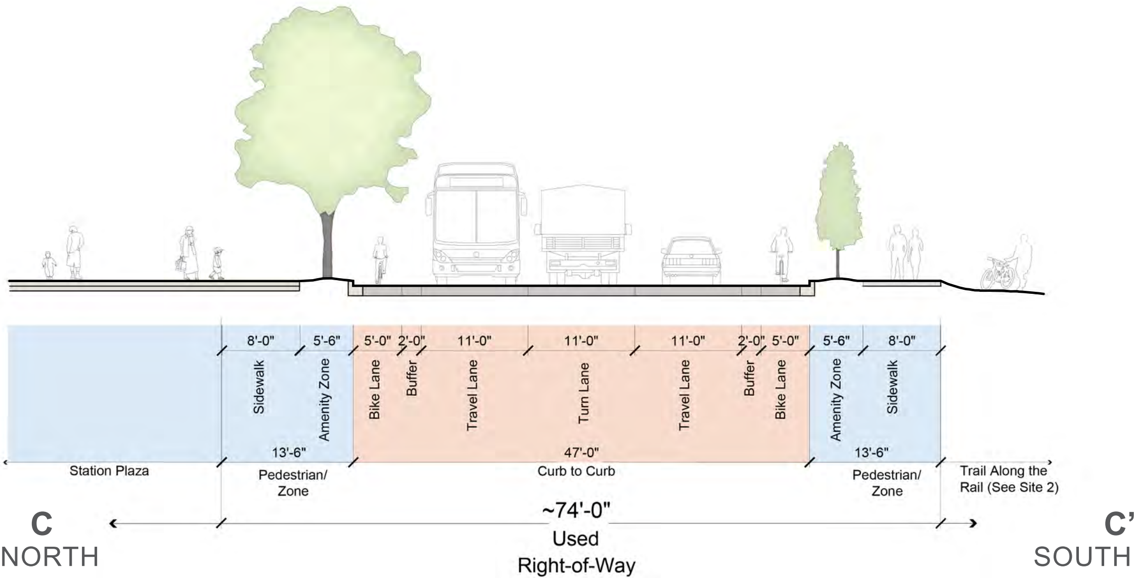
SECTION C FUTURE CONDITIONS (SOUND TRANSIT)
