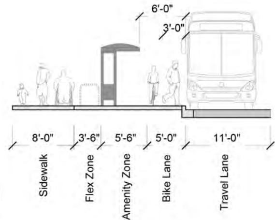
SECTION B OPTION 1 AT TRANSIT STOP
