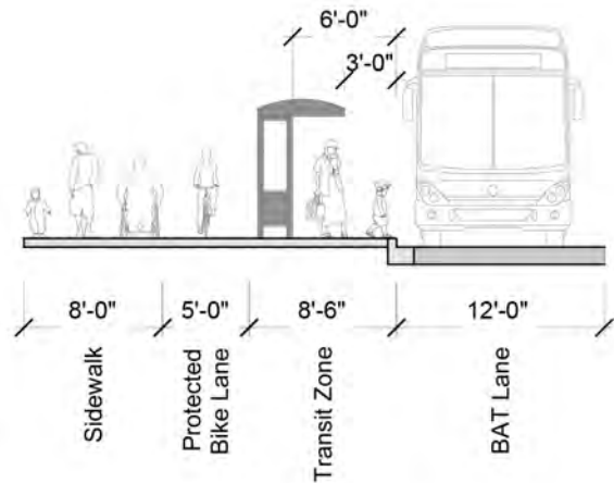
SECTION B OPTION 2 AT TRANSIT STOP
