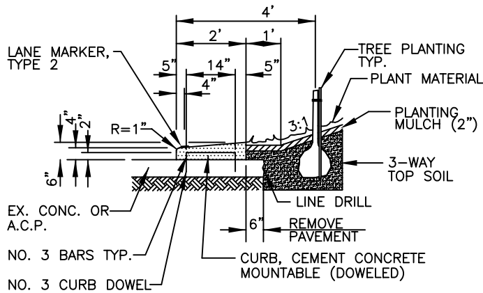
TYPICAL SECTION A
