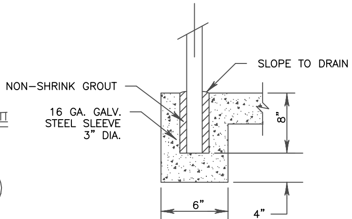
POST DETAIL
