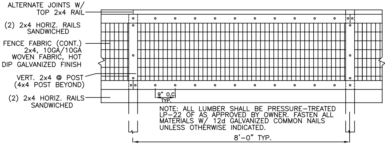
ELEVATION NOTE: HEIGHT VARIES, SEE CHAPTER 3, ENGINEERING DEVELOPMENT GUIDE
