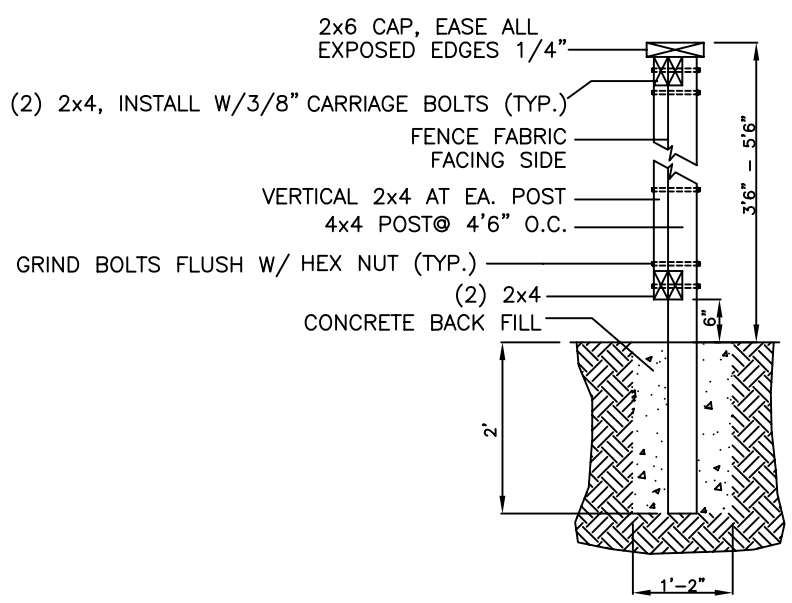
SECTION
