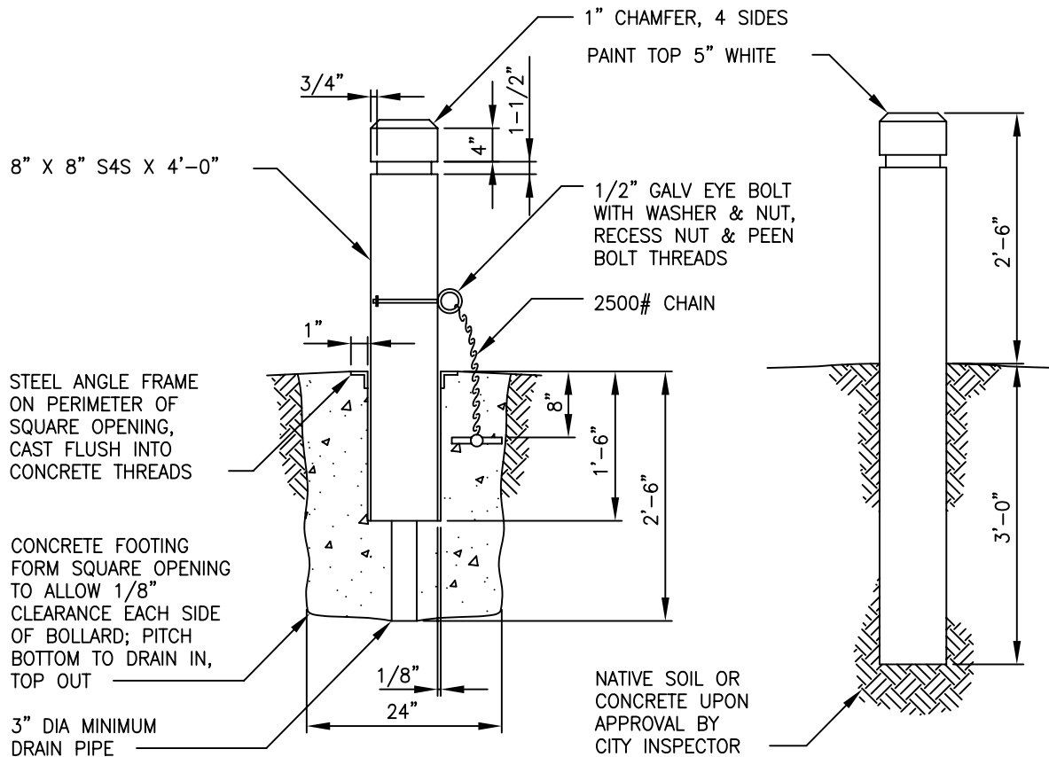
REMOVABLE BOLLARD
