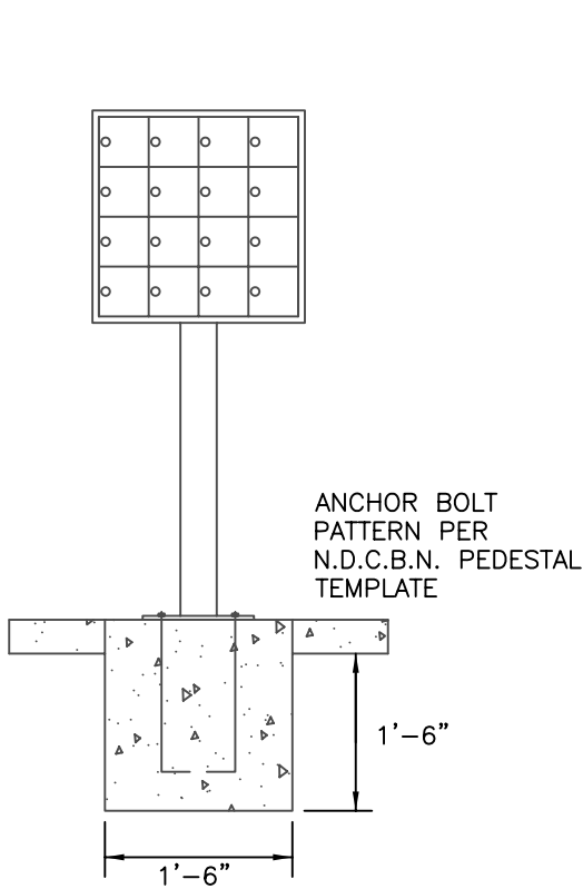
FRONT VIEW
