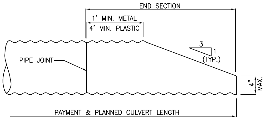
METAL & PLASTIC PIPE
