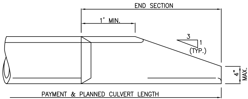
ELEVATION CONCRETE PIPE
