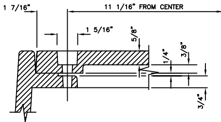
BOLT-DOWN DETAIL
