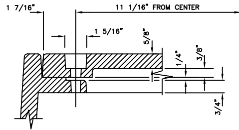
BOLT-DOWN DETAIL
