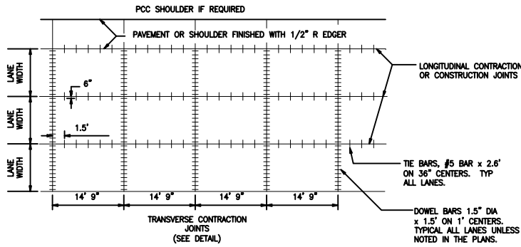
CEMENT CONCRETE PAVEMENT - DOWEL BAR JOINTS
