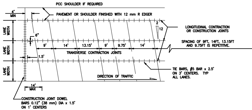
CEMENT CONCRETE PAVEMENT - PLAIN JOINTS
